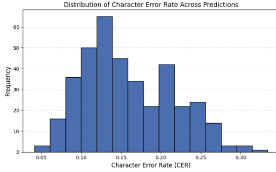
Figure B.1: Distribution of Character Error Rate (CER) across lexical restoration predictions.
