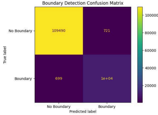
Figure 4.4: Confusion matrix for Sandhi boundary prediction.
