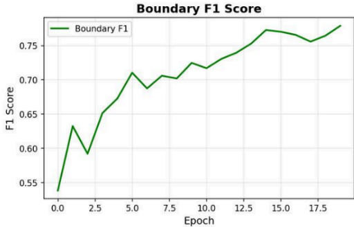
Figure 4.2: Boundary detection F1-score progression across training epochs.
